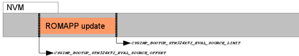
Figure 312.2. Application Update image
