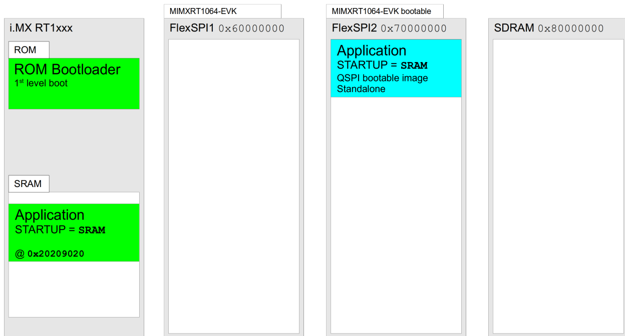
Figure 318.1. Standalone mimxrt1064_evk SRAM application
